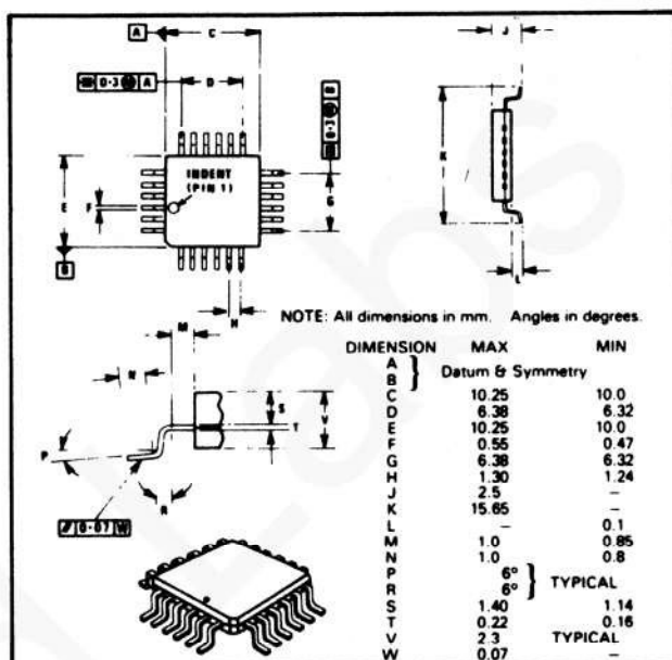
Fig.7 FX013LG quad plastic Package
