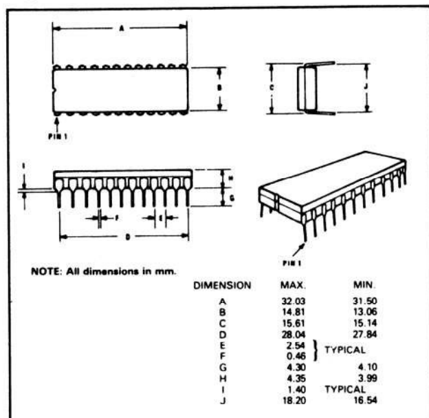
Fig.6 FX013J 24-pin cerdip Package
