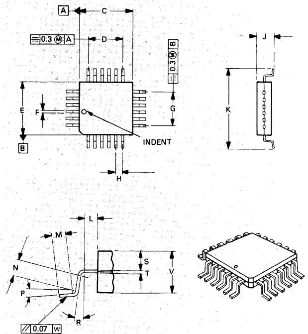
Fig. 9 FX409LV1 Package
