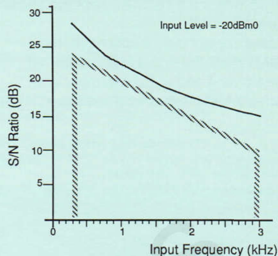
Fig.11 S/N vs Input Frequency (32kbit/s)
