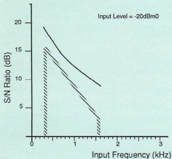
Fig.10 S/N vs Input Frequency (16kbit/s)
