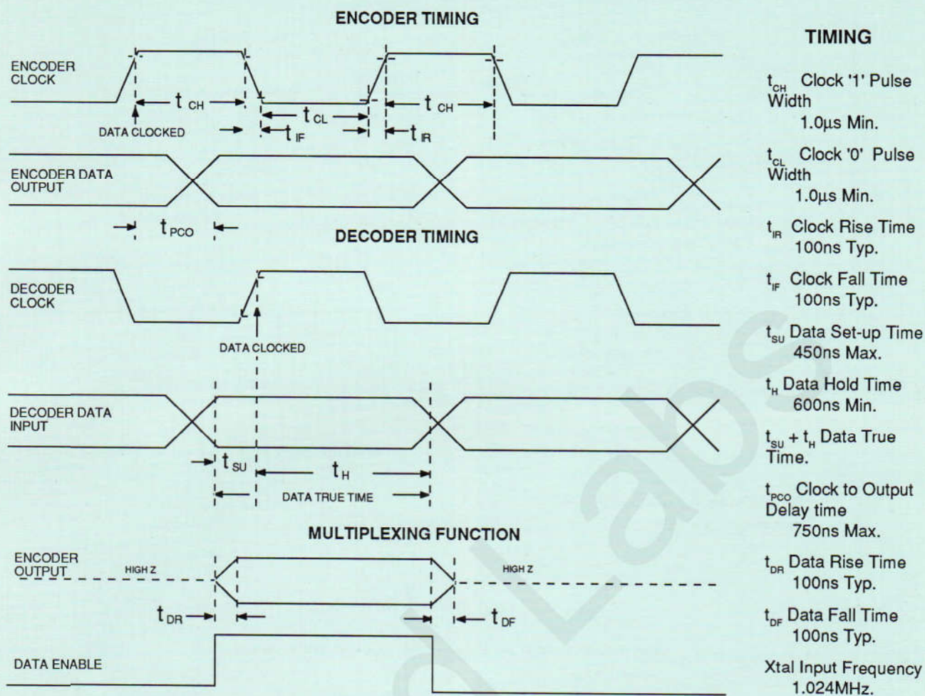
Fig.4 Codec Timing Diagrams
