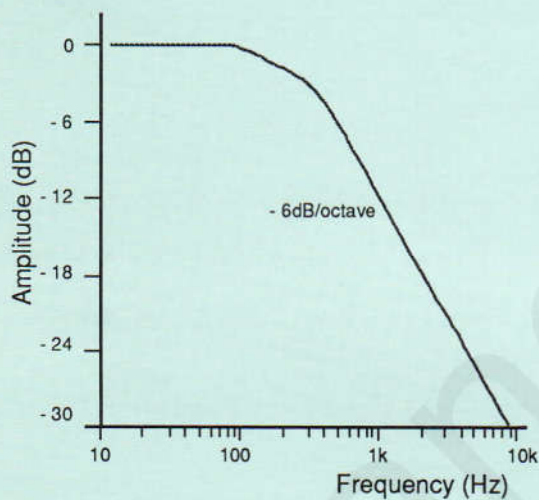
Fig.12 Principal Integrator Response
