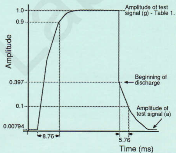
Fig.13 Compand Envelope
